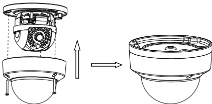
Figure 2-7 Bubble Reinstallation
