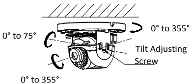
Figure 2-6 Type II Camera 3-Axis Adjustment
