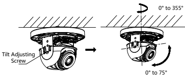
Figure 2-5 Type I Camera 2-Axis Adjustment
